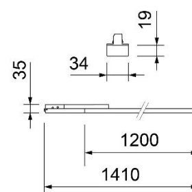
Version 1200mm
