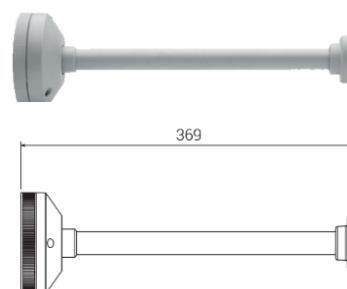
Clock Montagearm
