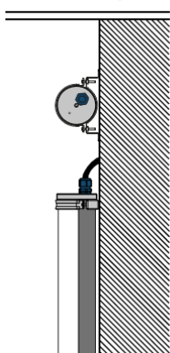
Wandmontage
