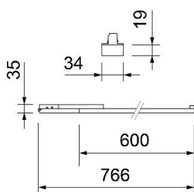
Version 600mm
