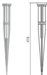
Clock Gartenspiess
