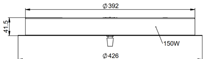
Baldachin 1x150W / 2x150W
