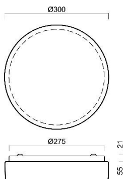
DELIA 1
